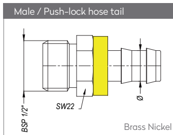
Male / Push-lock hose tail
